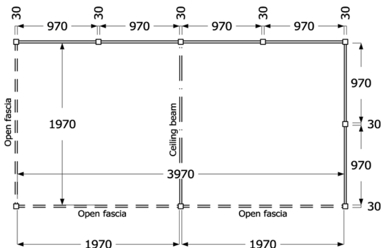
Example Technical Plan Layout
